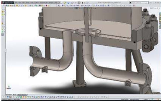
3D Design for System Integration
